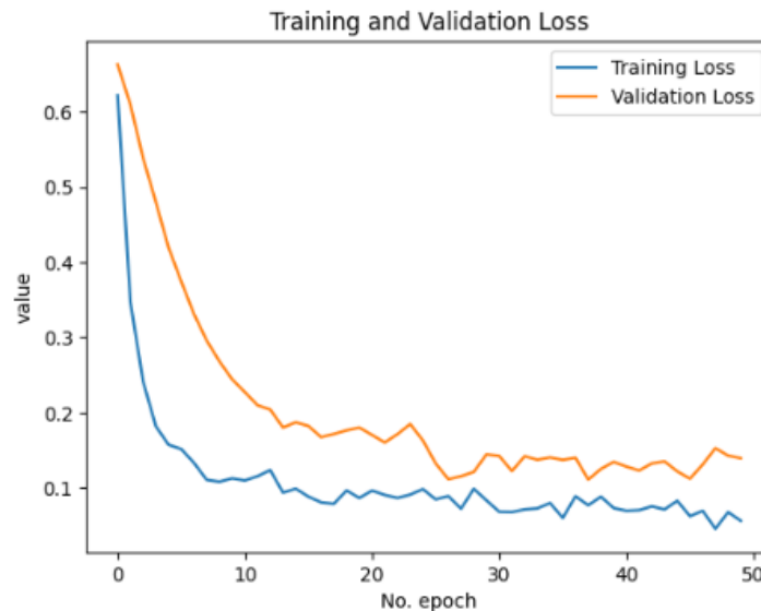
Gambar 1. Training and Validation Loss
